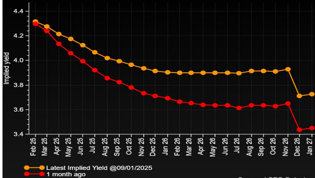
Implied Yield for CBOT 30-Day Fed Funds Futures Curves
